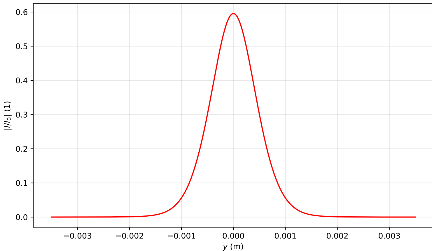
Intensity profile I(x=0, y, z=2.866)/I_0 , P_{in}=0.5P_{cr} , artificial time
